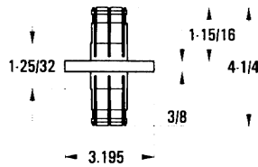
3-1/8" EIA
