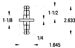
1-5/8" EIA
